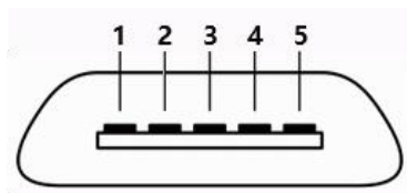
Micro-USB Female
